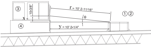
D3 — Elevation View
