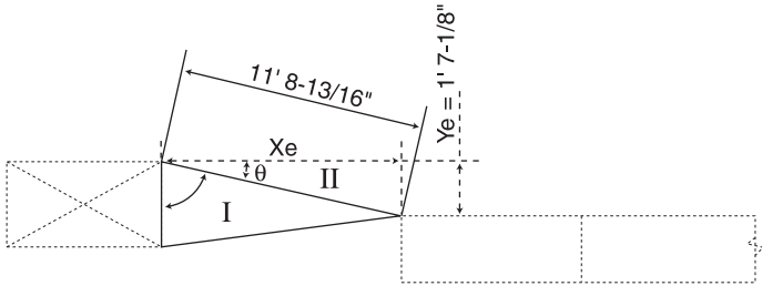
D2 — Elevation View Vertical Dimension
