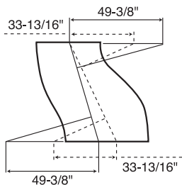
Centerline Layout "RAD"
