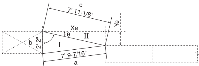
D1 — Elevation View Vertical Dimension
