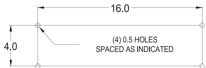
MOUNTING BOLT PATTERN
